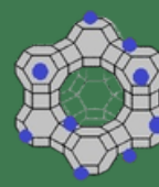
Zeolite
