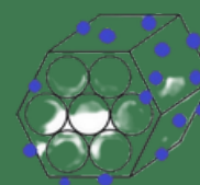
MCM-41
