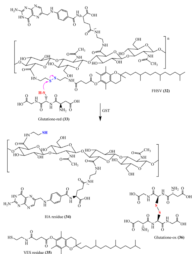
Figure 10. Mechanism for reducing disulfide binding 65,67
