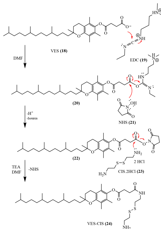
Figure 7. VES-CYS synthesis 42
