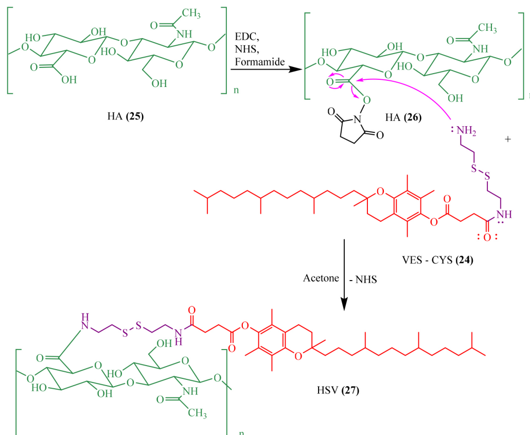
Figure 8. HSV synthesis 42
