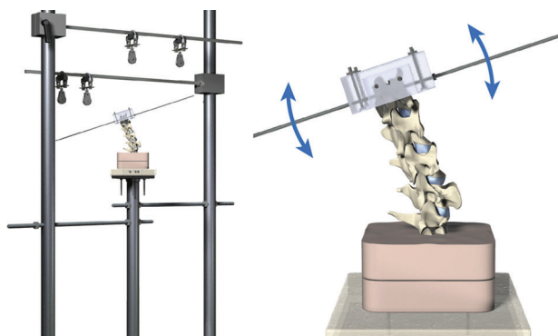
Figure 2 C3–T1 specimen in the neutral position loaded into a custom-designed testing apparatus (0.0 Nm).
